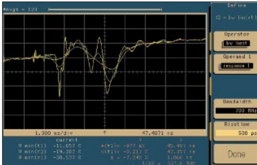
Figure 2. The measurements of input impedance of PHY #1 TPB Port were obtained using the amplitude of reflection method.
