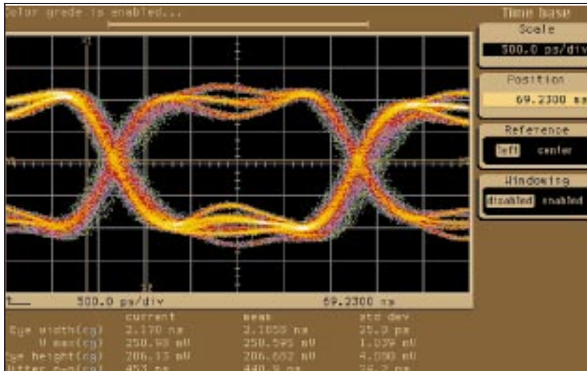
Figure 3. The digitizing oscilloscope performs automatic measurements and displays the jitter in the left-hand corner of the screen. This is the jitter of a failing S400 PHY.
