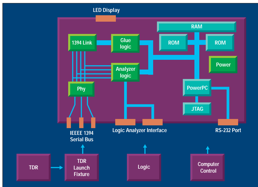
Figure 1. The basic components of the IEEE 1394 TDR test setup.
